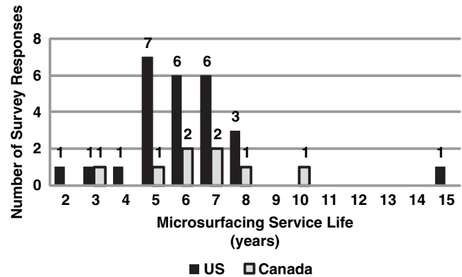
FIGURE 5 Summary of survey microsurfacing service life responses.
